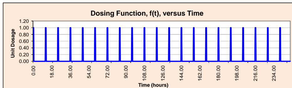
Figure 5: A graph of the dosing function f(t) versus time.
