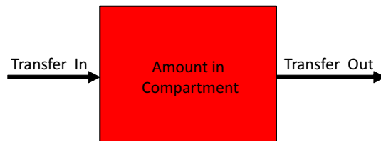
Figure 3: A generic one compartment model.
