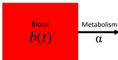
Figure 2: A compartment representation of a single injection model.
