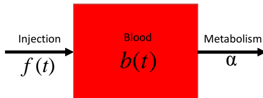
Figure 1: A compartment representation of a multiple injection model.
