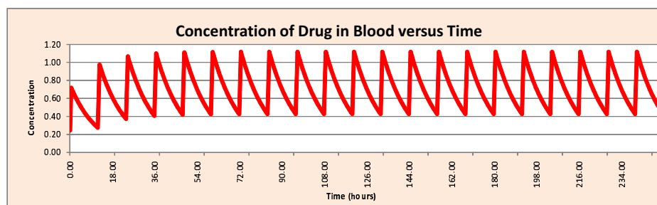
Figure 6: A graph of b(t) versus time for the multiple injection model.
