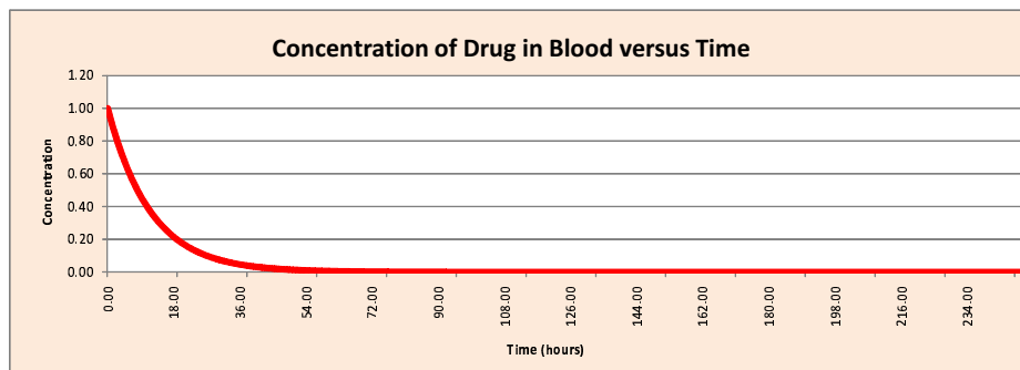
Figure 4: A graph of b(t) versus time for the single injection model.
